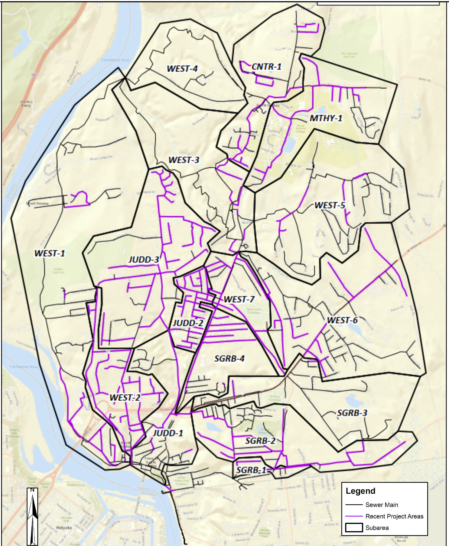
Figure 10 Sewersheds
