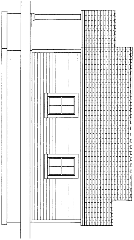
RIGHT ELEVATION 1/4"=1'0"
